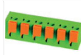
DG142V-7.62 VDE 450V/15A 0.2-1.5mm 2 UL 300V/10A 22-16AWG Pola/Poles 1P-XXP
