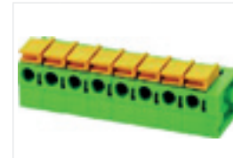
DG142R-5.08 VDE 250V/15A 0.2-1.5mm 2 UL 300V/10A 22-16AWG Pola/Poles 1P-XXP
