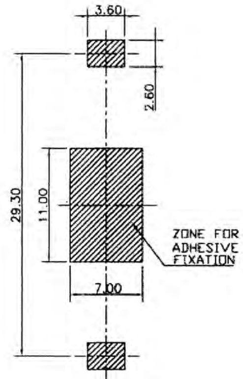
PCB LAYOUT
