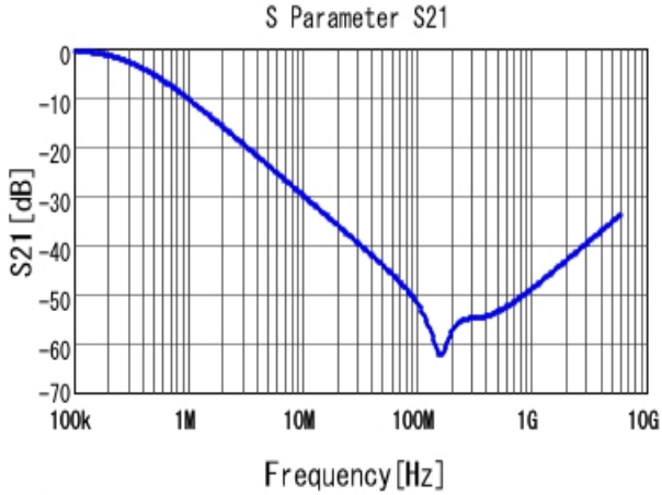
■ NFM18CC223R1C3 S21 DC0V, 25degC, Feedthrough
