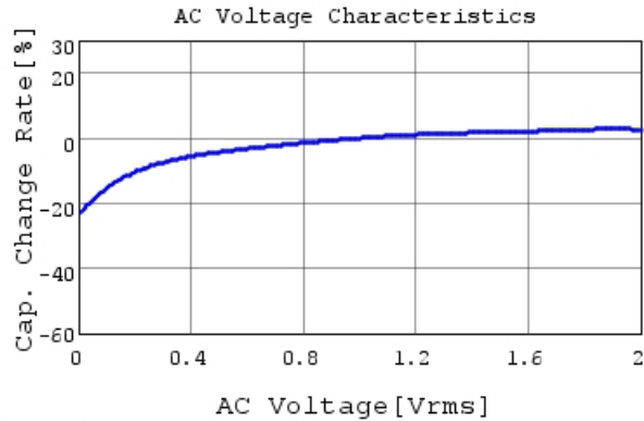
GRM155R61C225KE11 C-AC Voltage capchange, DC
