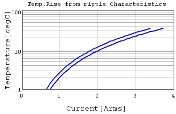
GRM155R61C225KE11 Temp.rise — 500kHz
