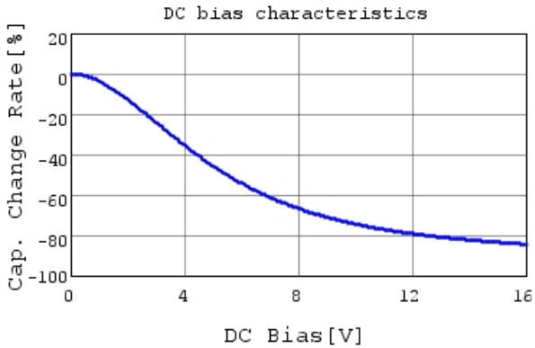
GRM155R61C225KE11 C-DC bias capchange, 25.0c
