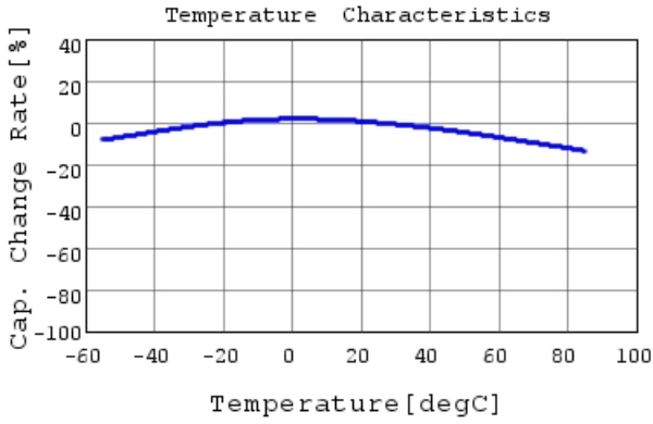
GRM155R61C225KE11 C-Temp. capchange, DC0.0V,
