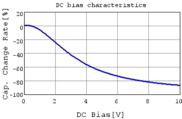
GRM31CR61A107MEA8 C-DC bias capchange, 25.0c
