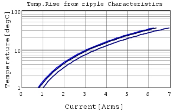
GRM31CR61A107MEA8 Temp.rise — 50kHz
