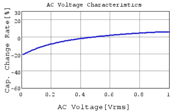
GRM31CR61A107MEA8 C-AC Voltage capchange, Dc
