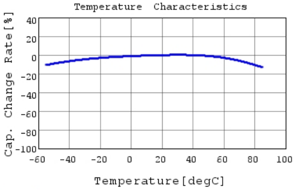
GRM31CR61A107MEA8 C-Temp. capchange, DC0.0V,
