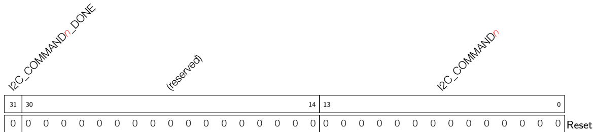
Register 11.21: I2C_CMD n _REG ( n : 0-15) (0x58+4* n )
