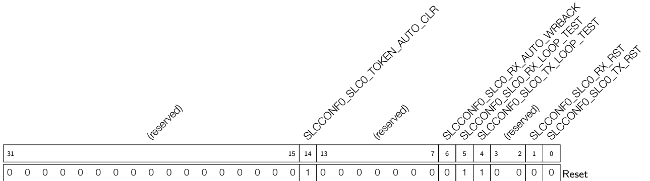
Register 8.1: SLCCONF0_REG (0x0)
