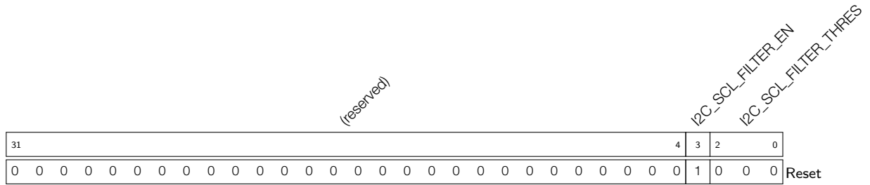
Register 11.19: I2C_SCL_FILTER_CFG_REG (0x0050)
