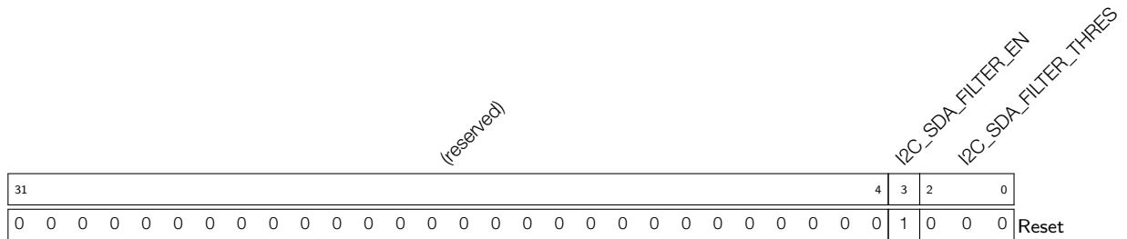
Register 11.20: I2C_SDA_FILTER_CFG_REG (0x0054)
