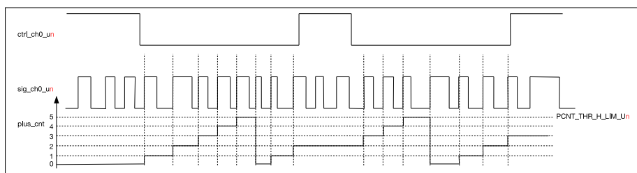
Figure 122: PULSE_CNT Upcounting Diagram
