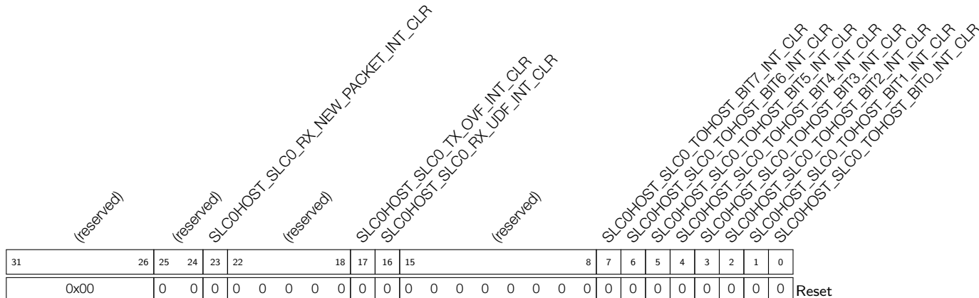
Register 8.33: SLC0HOST_INT_CLR_REG (0xD4)
