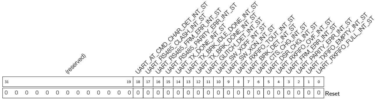
Register 13.3: UART_INT_ST_REG (0x8)
