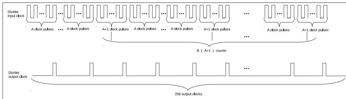
Figure 87: LED_PWM Divider
