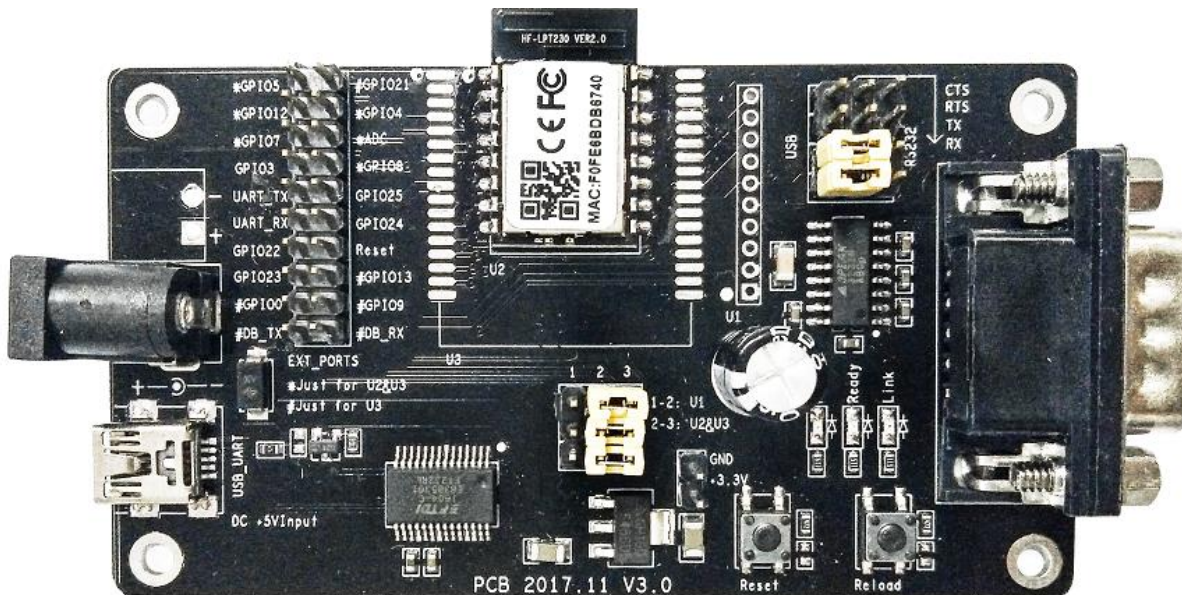
Figure 23. HF-LPT230 EVK
