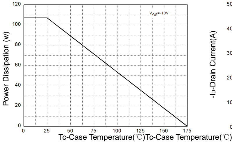
Figure 1: Power Dissipation
