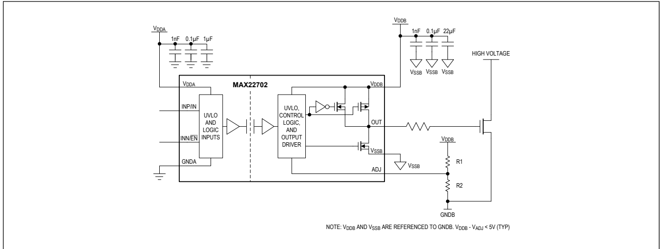
Figure 11. Example Circuit for MAX22702 Adjustable UVLO
