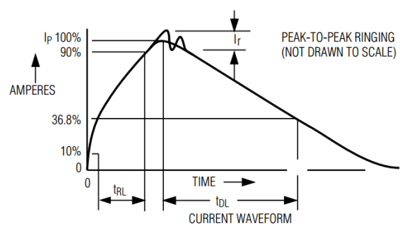
Figure 5 human body mode current waveform
