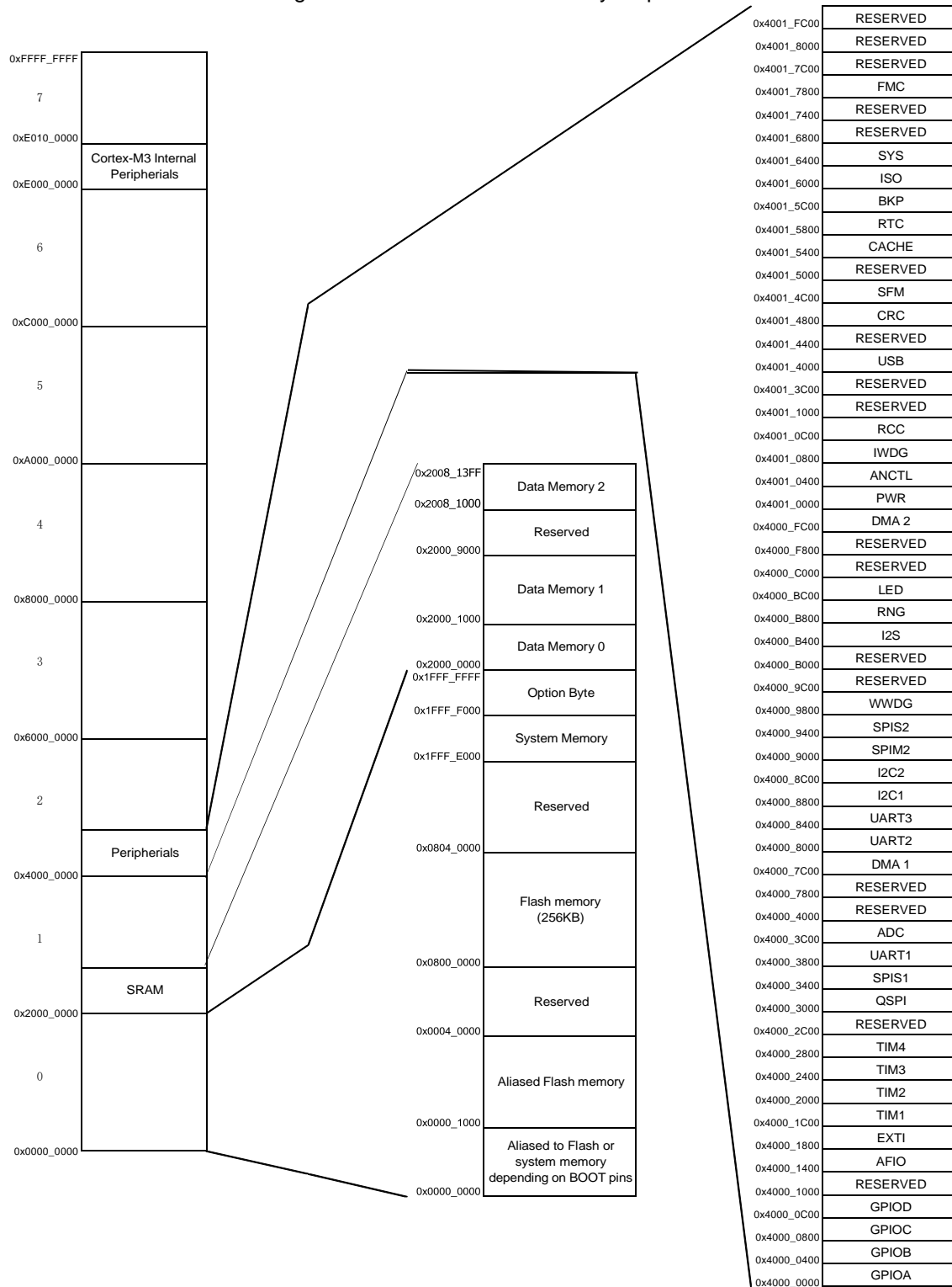
Figure 4.1: MG32F104xx memory map
