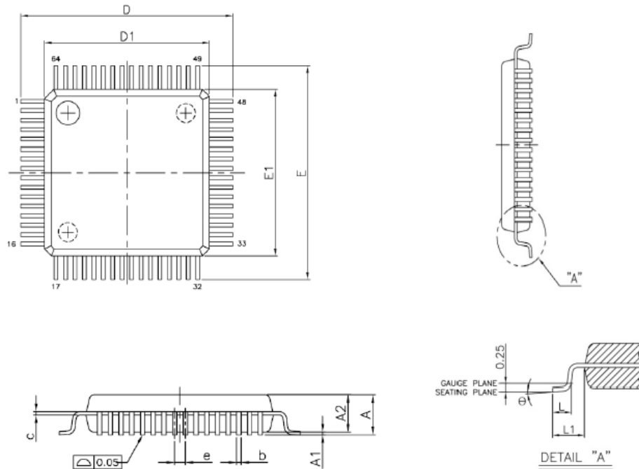
Figure 6.3: LQFP64 7X7mm, 0.4mm pitch and Recommended footprint
