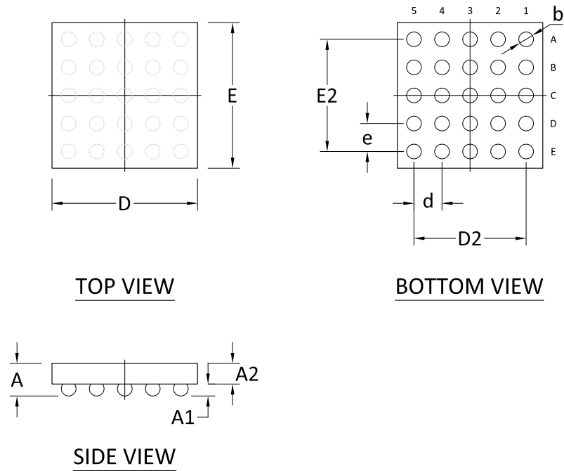
Figure 36: WLCSP 2.075x2.075 mm package
