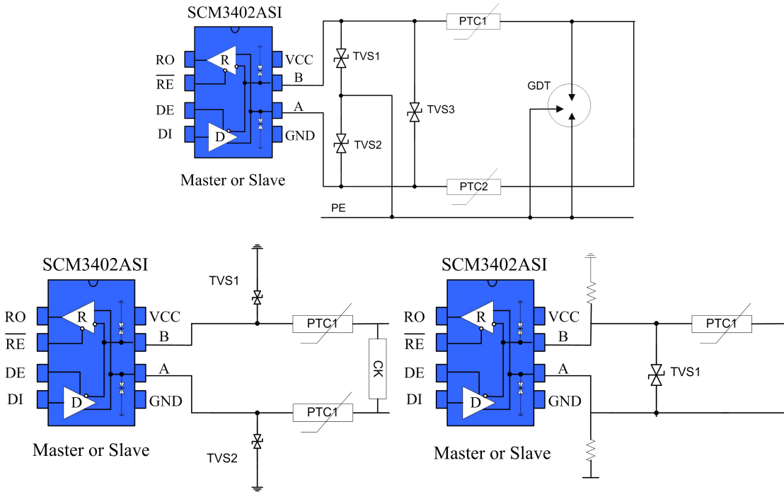
Figure 12. Port safeguard scheme
