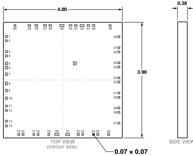
Figure 3. 50-Pad Bare Die [CHIP] (C-50-1) Dimensions shown in millimeters
