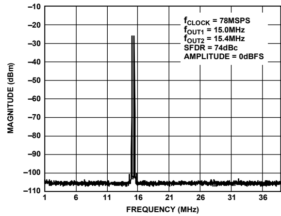
Figure 42. Dual-Tone SFDR
