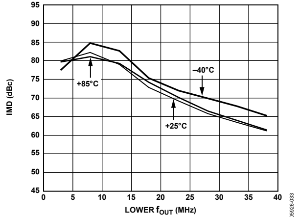
Figure 36. Dual-Tone IMD vs. Lower f_{OUT} and Temperature at 80 MSPS, I_{OUTFS} = 1 mA and 0 dBFS
