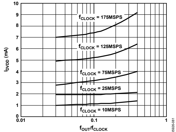
Figure 82. I_{DVDD} vs. f_{OUT}/f_{CLOCK} Ratio at DVDD = 3.3\text{ V}
