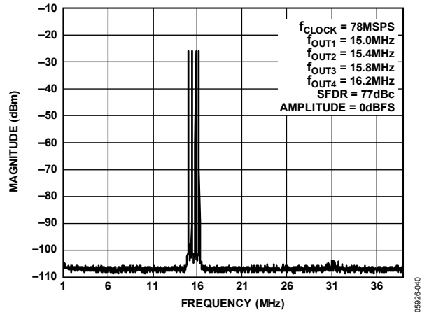
Figure 26. Four-Tone SFDR
