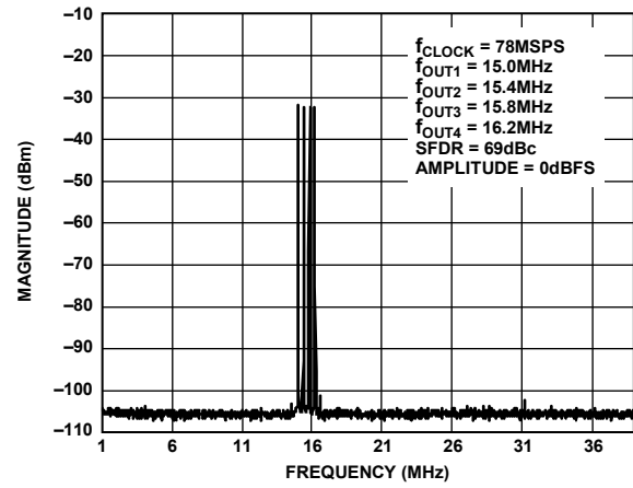
Figure 43. Four-Tone SFDR
