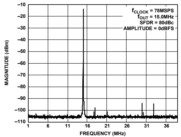
Figure 24. Single-Tone SFDR
