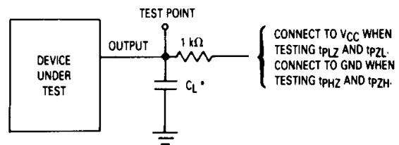
Figure 8. Test Circuit
