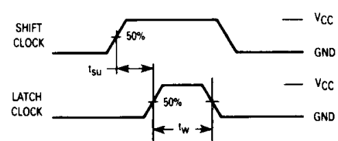
Figure 6. Switching Waveforms
