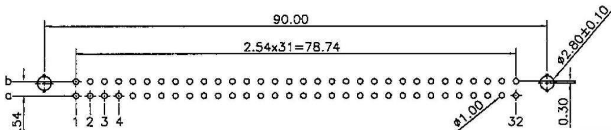
P.C. Board Layout
