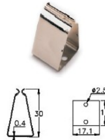
BH980-3 HOLDER
