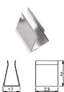
BH980 HOLDER
