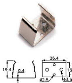
BH980-2 HOLDER
