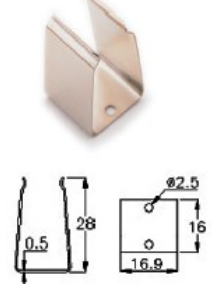
BH980-4 HOLDER
