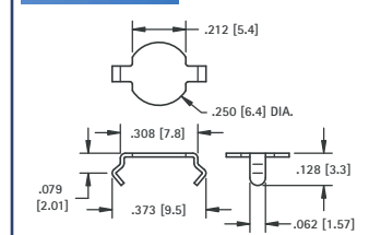
Mounting Detail
