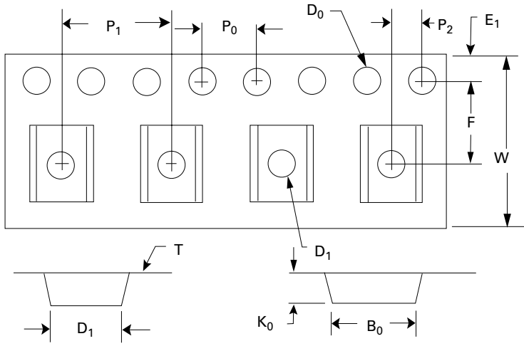
Tape Specifications
