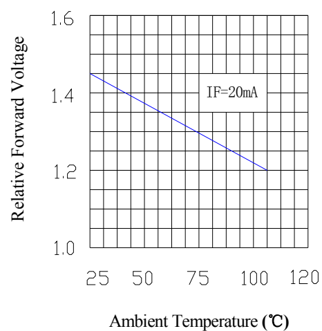
Forward Voltage & Ambient Temperature
