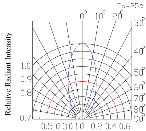
Relative Radiant Intensity & Angular Displacement
