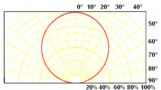
Directive Characteristics (Ta=25)
