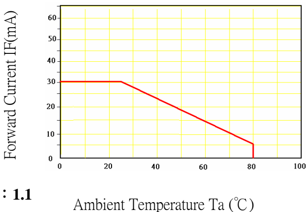
Fig.5 IF-Ta
