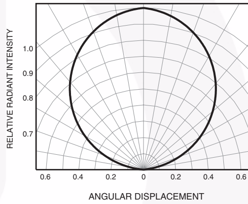
Fig. 8 Radiation Diagram
