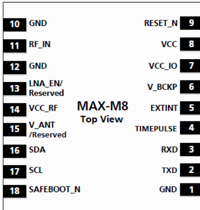
Figure 2: Pin Assignment
