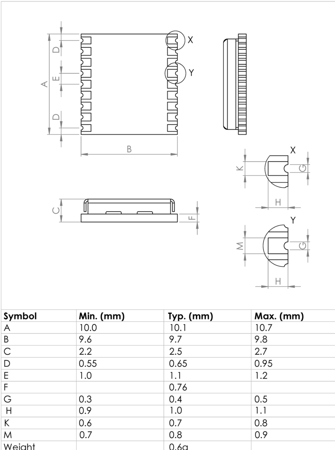
Figure 3: Dimensions
