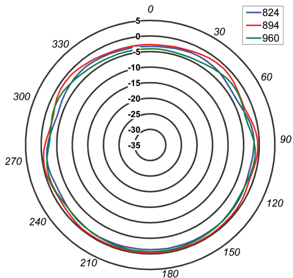
E Plane
