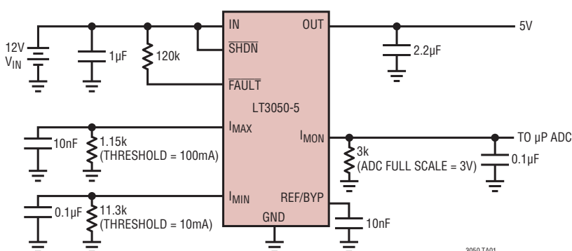
5V Supply with 100mA Precision Current Limit, 10mA I_{MIN}
