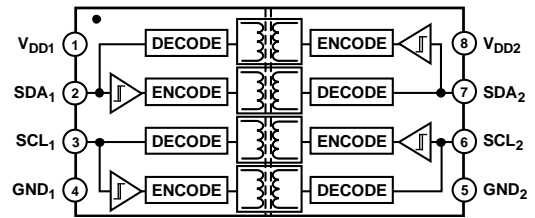
Figure 1. ADuM1250
