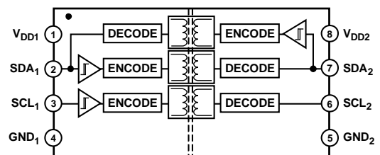
Figure 2. ADuM1251
