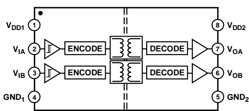
Figure 1. ADuM3200 Functional Block Diagram
