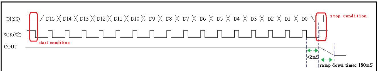
Fig. 17 Power-Down command timing
