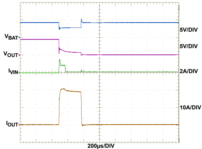
FIGURE 10. V_{OUT} SHORTED WITH BATTERY CONNECTED
