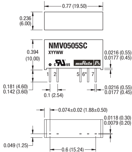
SIP package
