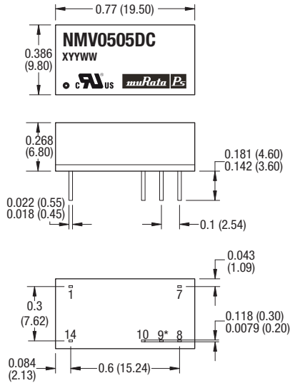
DIP package
