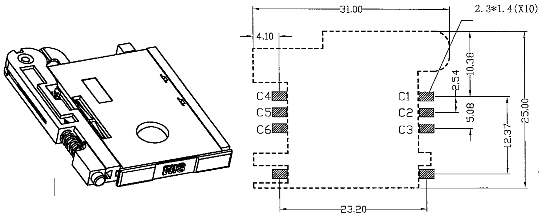
Unit :mm;Tolerances :±0.20mm Mechanical outline dimension
