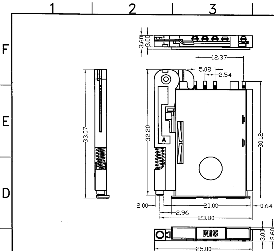
Unit :mm;Tolerances :±0.20mm Mechanical outline dimension
