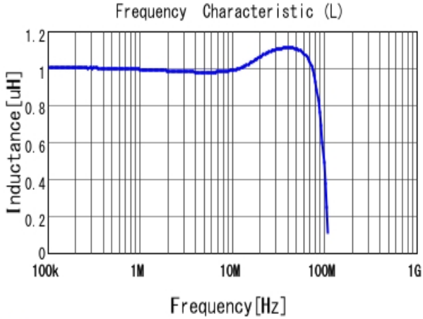
■ LQM21PN1R0MC0 L
