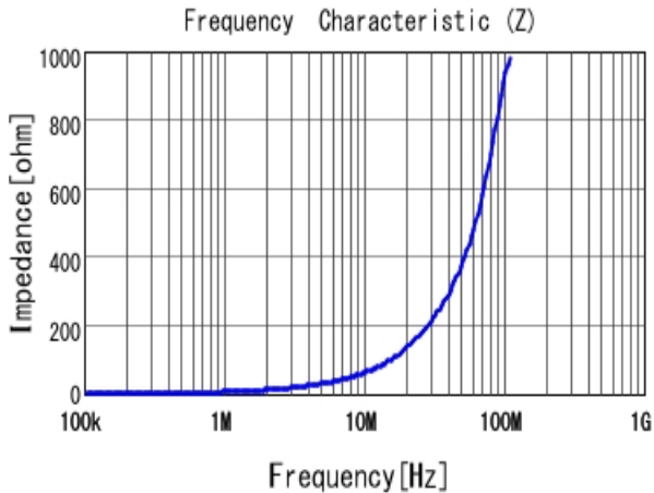
■ LQM21PN1R0MC0 |Z|
