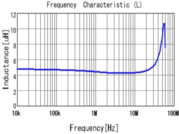
■ LQH44PN4R7MP0 L
