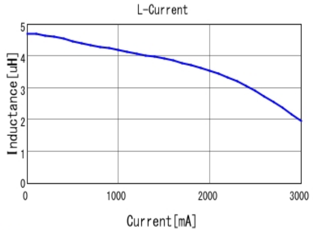
■ LQH44PN4R7MP0 L-Current 20degC
