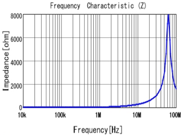
■ LQH44PN4R7MP0 |Z|
