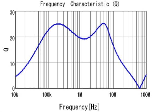
■ LQH44PN4R7MP0 Q
