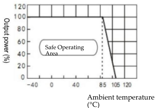
Temperature Curve
