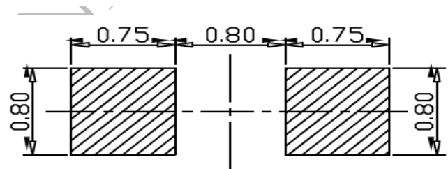
推荐焊盘尺寸 Recommended Soldering Pad
