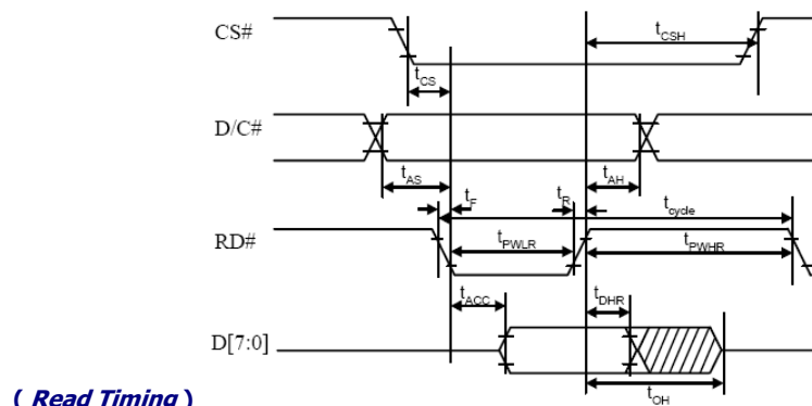
( Read Timing )
