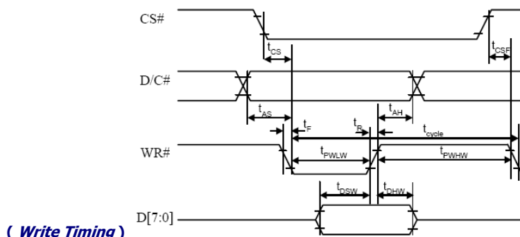
( Write Timing )
