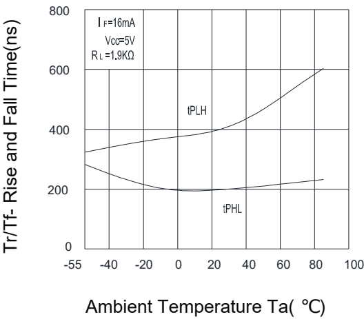
Fig.8 Propagation Delay Time vs. Ambient Temperature
