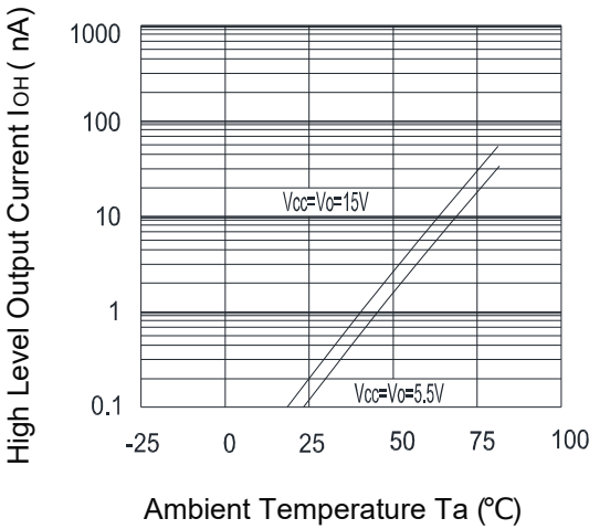
Fig.7 High Level Output Current vs. Ambient Temperature
