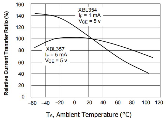
Figure 6. Relative Current Transfer Ratio vs. Ambient Temperature
