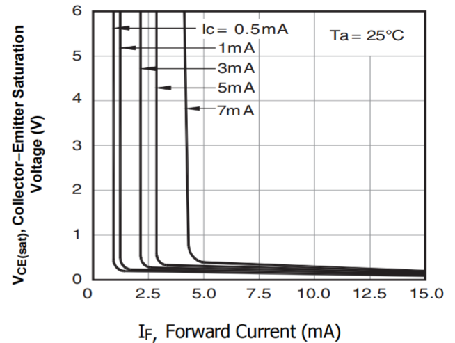
Figure 2. Collector-Emitter Saturation Voltage vs. Forward Current
