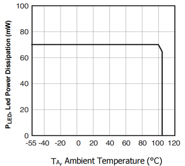
Figure 8 . Led Power Dissipation vs. Ambient Temperature
