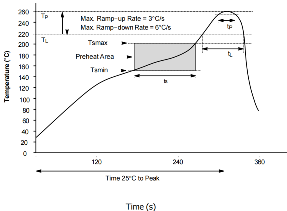
Figure 14. Reflow Profile
