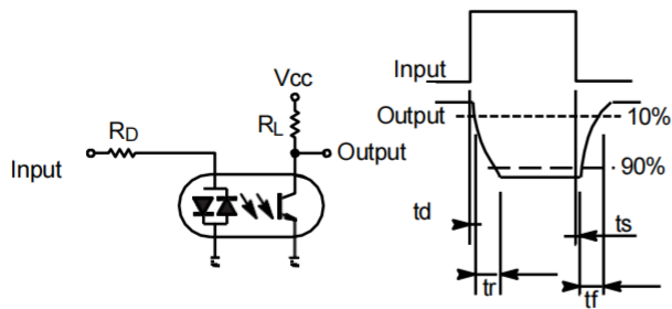
Figure 12. Test Circuit for Response Time
