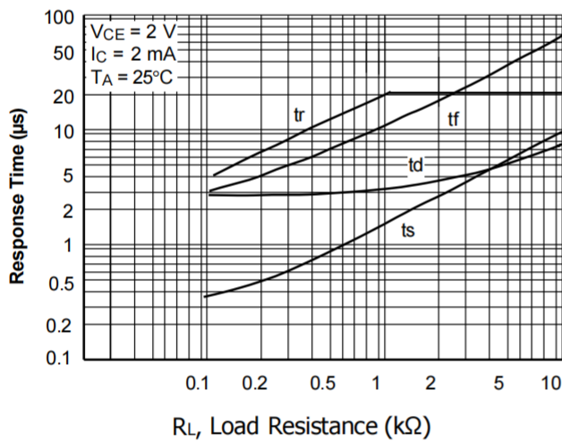
Figure 9 . Response Time vs. Load Resistance
