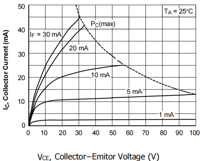
Figure 5. Collector Current vs. Collector-Emitter Voltage
