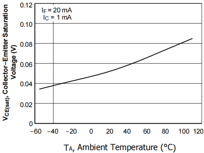
Figure 7 . Collector-Emitter Saturation Voltage vs. Ambient Temperature
