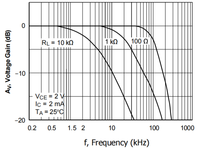
Figure 10 . Frequency Response
