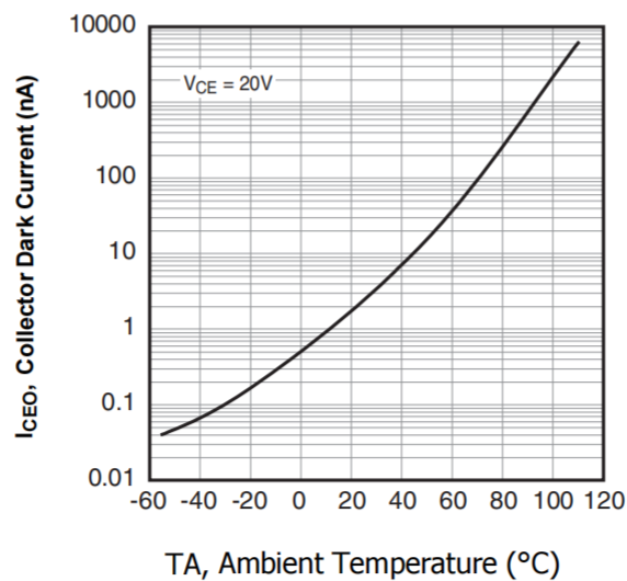
Figure 11. Collector Dark Current vs. Ambient Temperature
