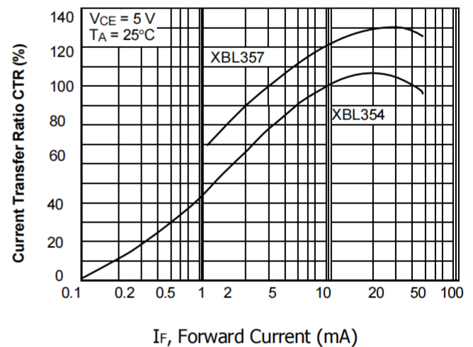
Figure 4. Current Transfer Ratio vs. Forward Current
