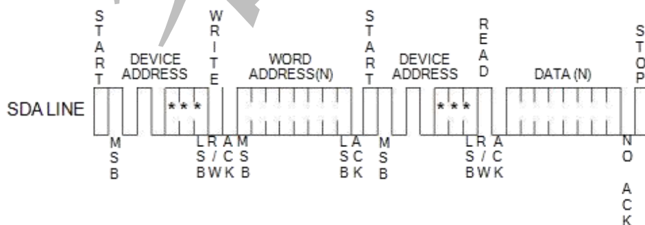
Figure 9: Random Read
