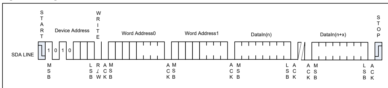
Figure 5-2 Page Write
