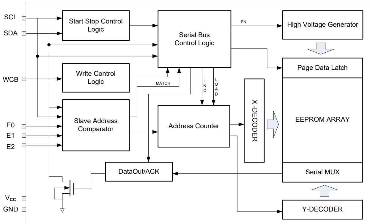
Figure 2-1 Block Diagram
