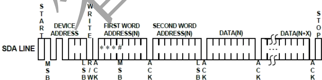
Figure 4: Page Write
