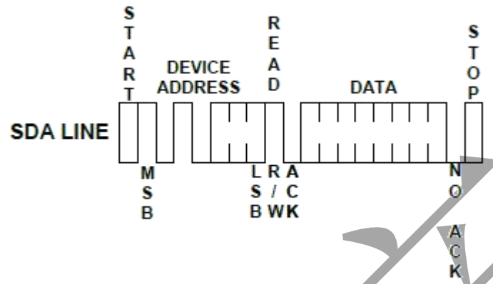
Figure 5: Current Address Read
