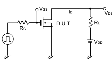
Fig.13 Switching time measurement circuit
