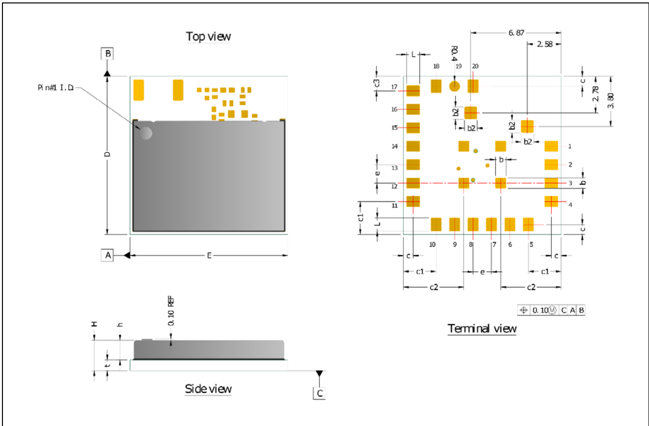
Figure 6. Package outline drawings
