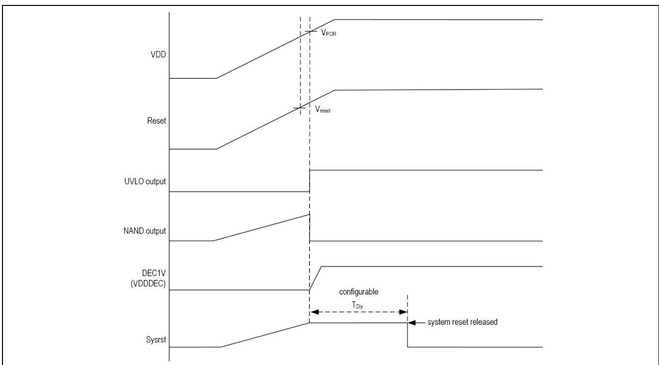
Figure 2. Power-up sequence
