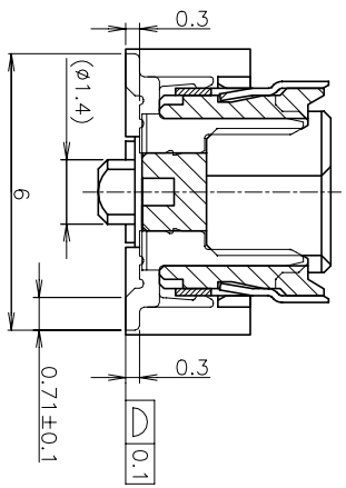
SECT. Z-Z (SIGNAL POSITION) (SCALE 8:1)
