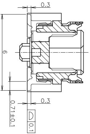
SECT. Y-Y (GROUND POSITION) (SCALE 8:1)
