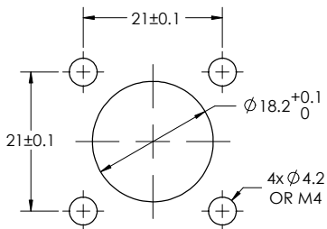
RECOMMENDED PANEL LAYOUT
