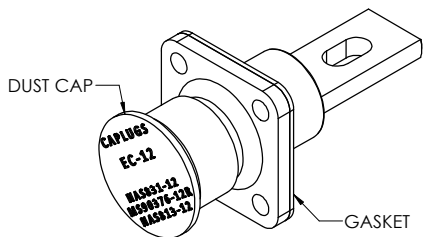
DUST CAP ASSEMBLY DIAGRAM
