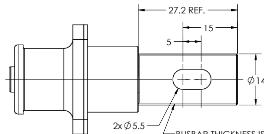
BUSBAR TYPE
