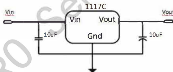
Application circuit of LD1117 fixed version
