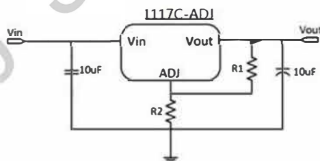
Application Circuit of LD1117-ADJ
