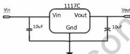
Application circuit of LD1117 fixed version
