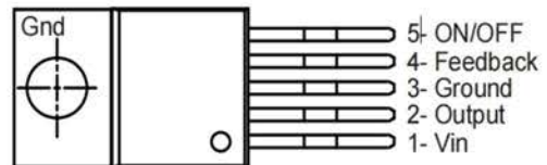
LM2576TB-XX
