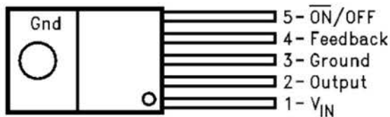
LM2576T-XX 或 LM2576HVT-XX
