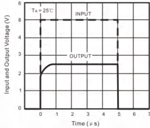
Pulse Response
