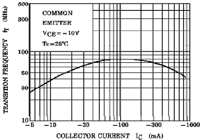
Fig 3: Transition Frequency vs Collector Current
