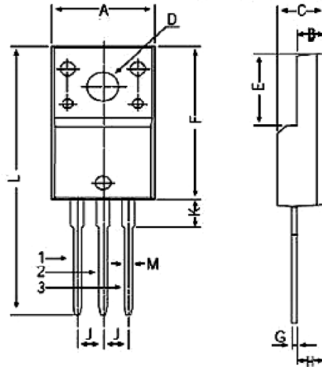
TO-220FP Leaded Plastic Package
